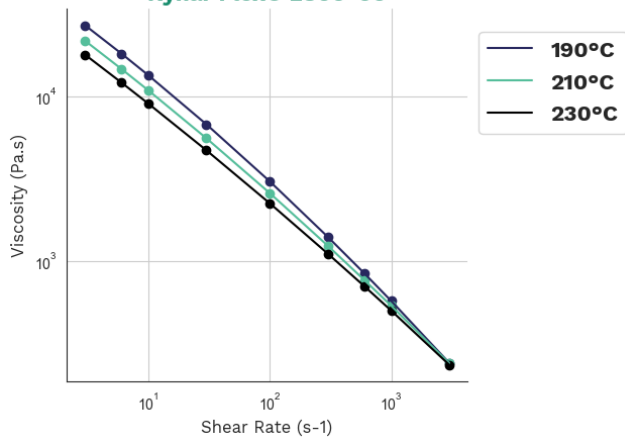
Viscosity-shear rate Kynar Flex® 2800-00
